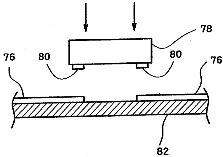
FIG. 9 PRIOR ART
